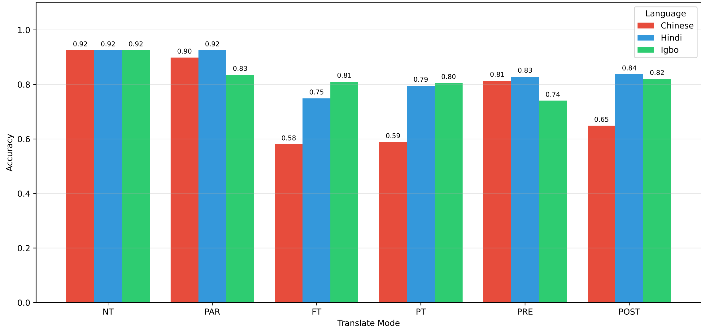
Granite-Small - Language Comparison
