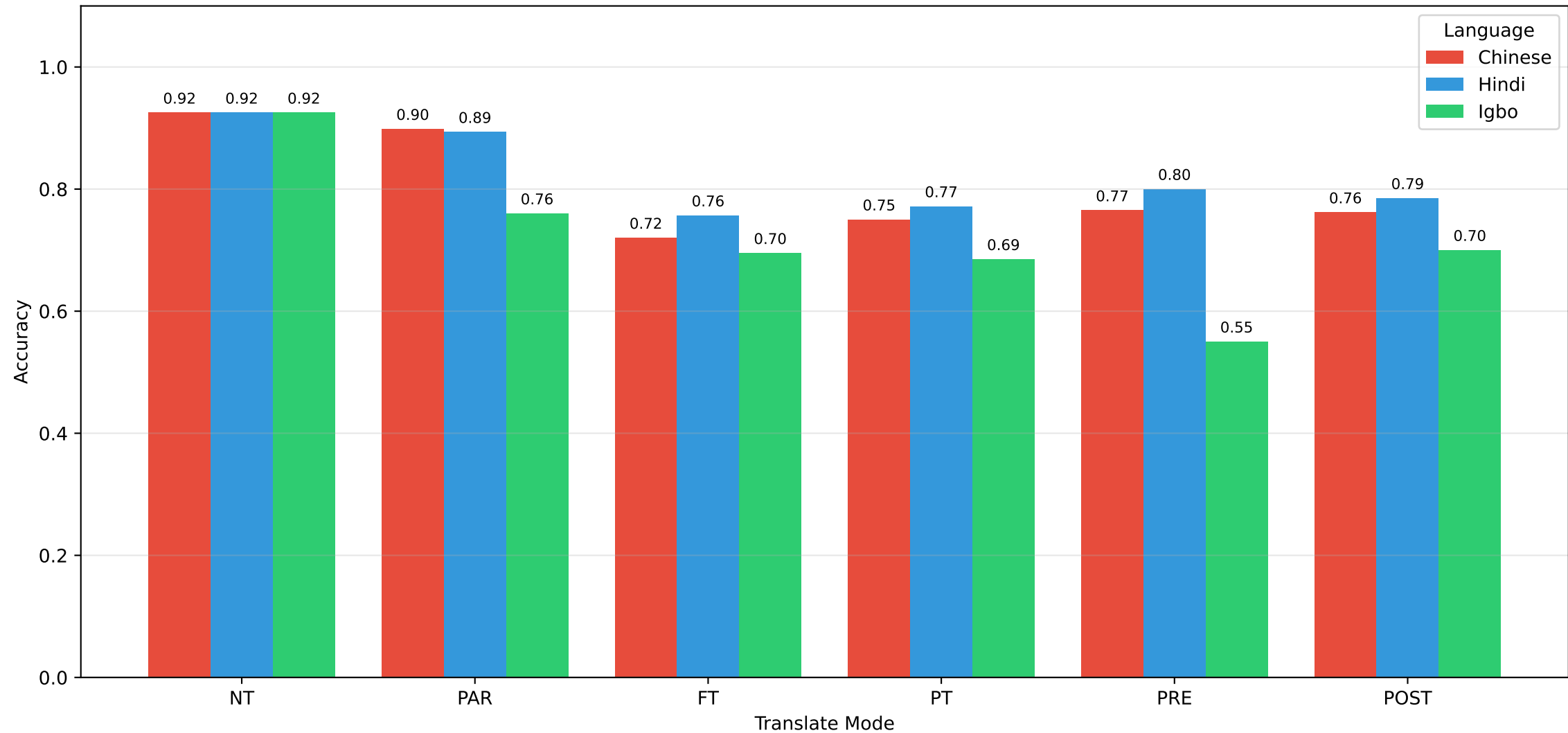
Granite-Tiny - Language Comparison
