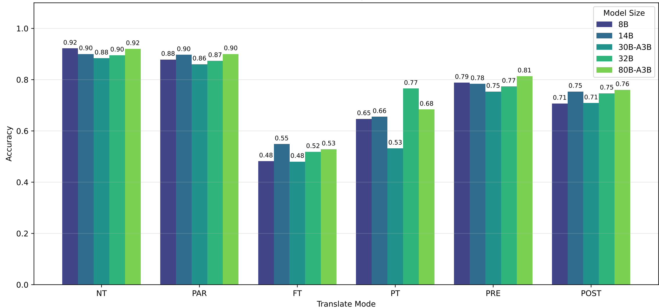
Qwen3 Model Size Comparison - Chinese
