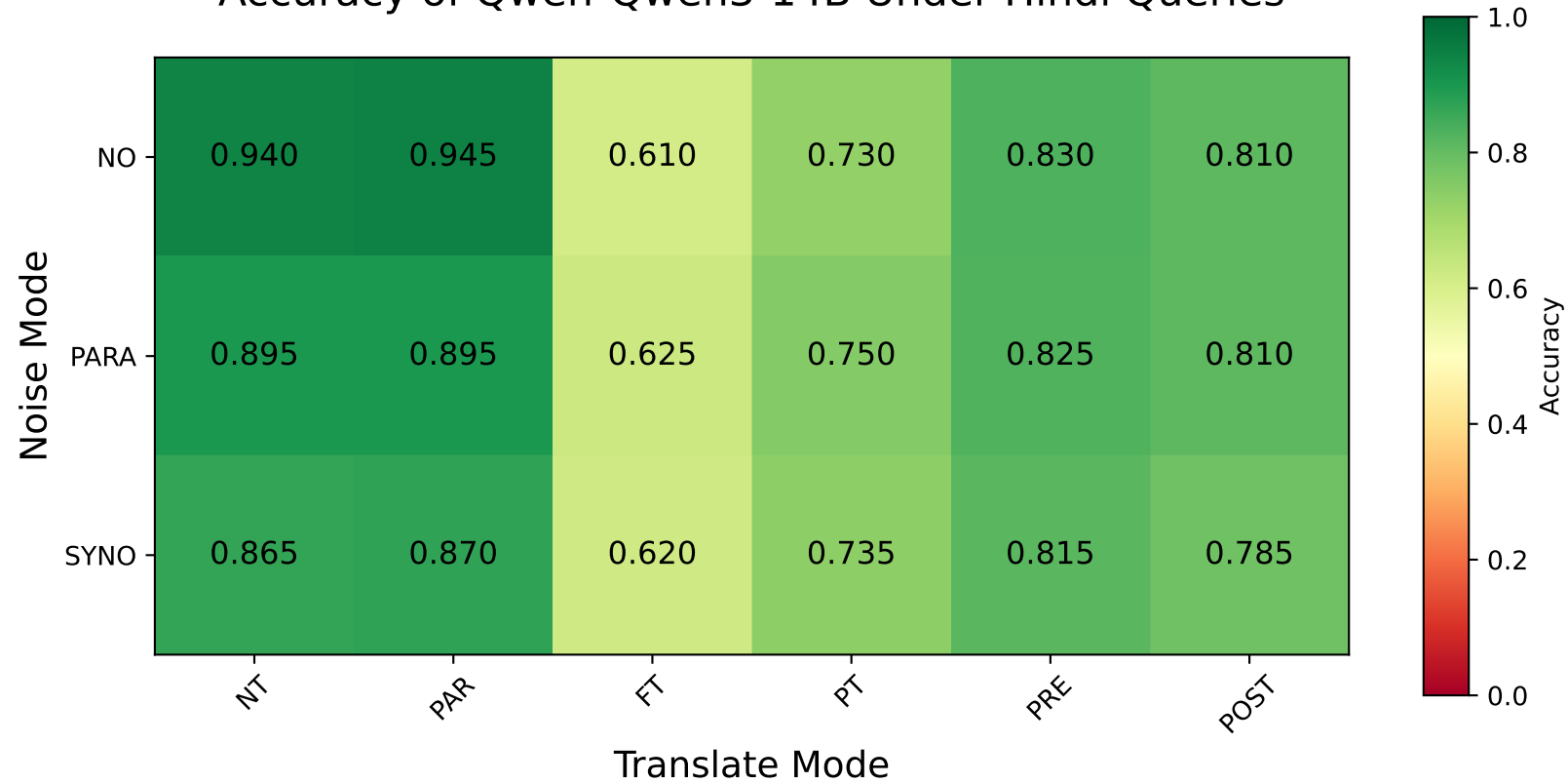
Accuracy of Qwen-Qwen3-14B Under Hindi Queries
