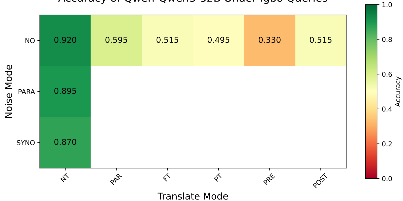
Accuracy of Qwen-Qwen3-32B Under Igbo Queries
