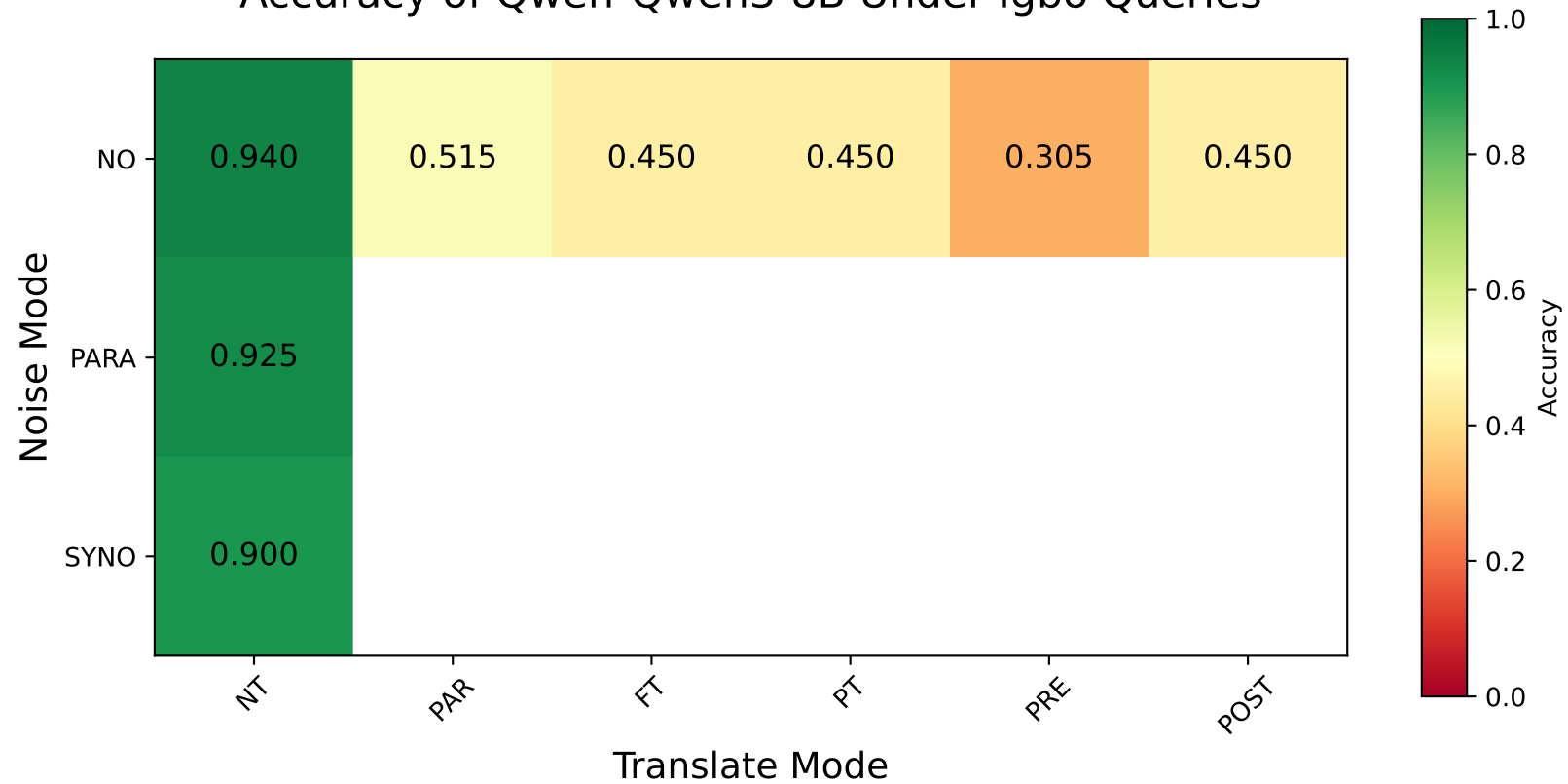
Accuracy of Qwen-Qwen3-8B Under Igbo Queries
