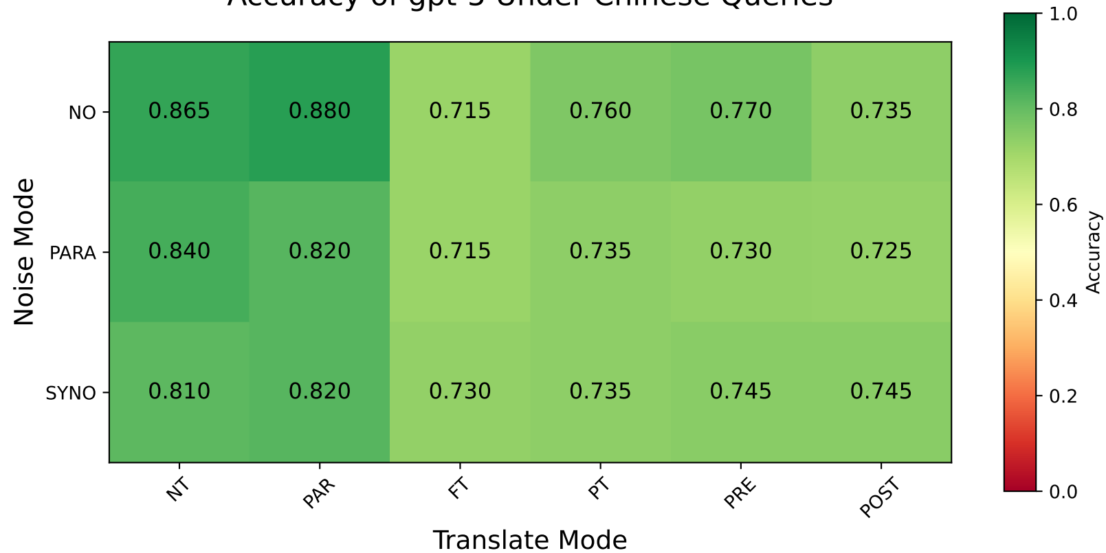
Accuracy of gpt-5 Under Chinese Queries
