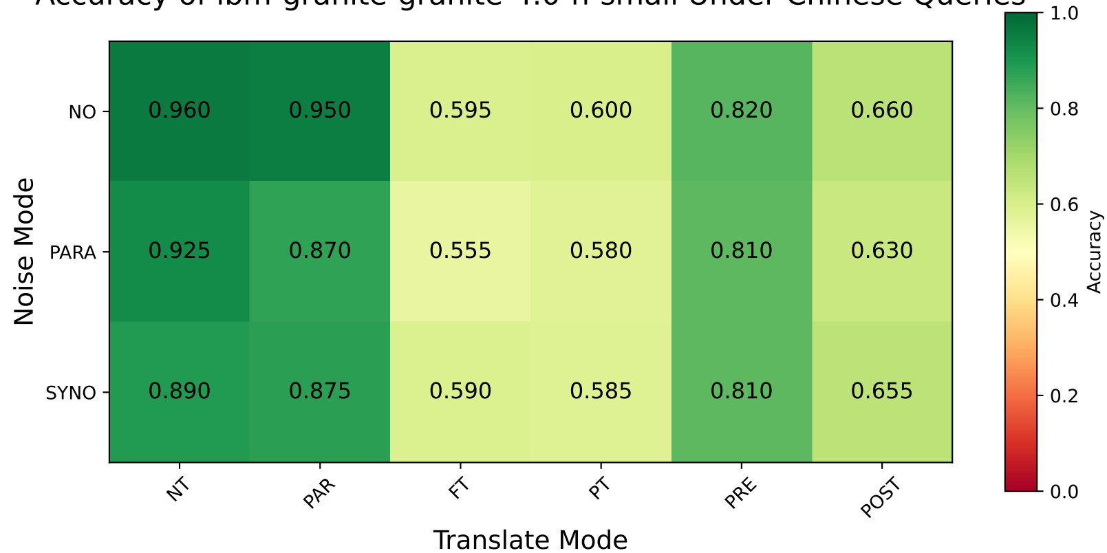
Accuracy of ibm-granite-granite-4.0-h-small Under Chinese Queries
