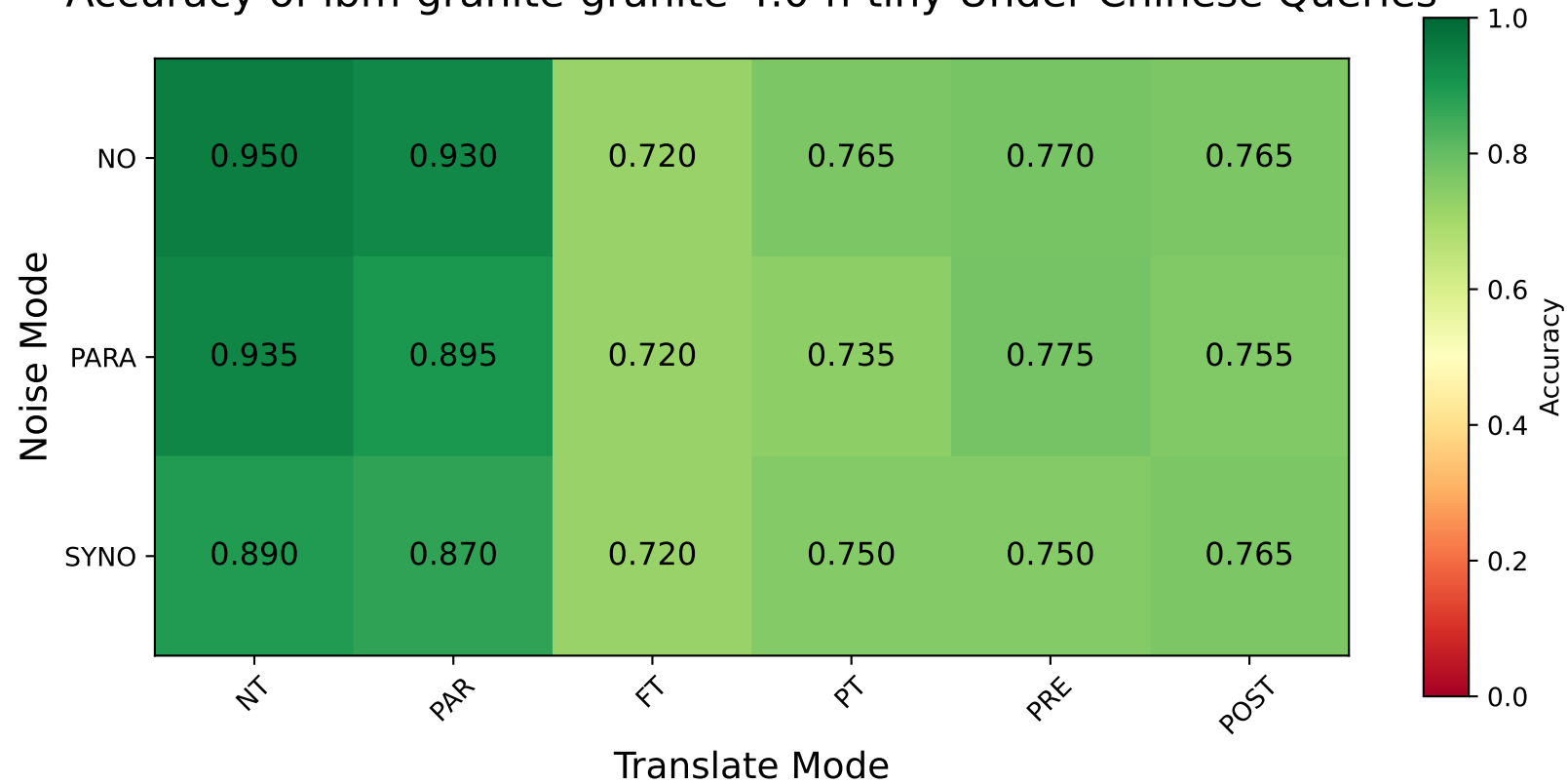
Accuracy of ibm-granite-granite-4.0-h-tiny Under Chinese Queries
