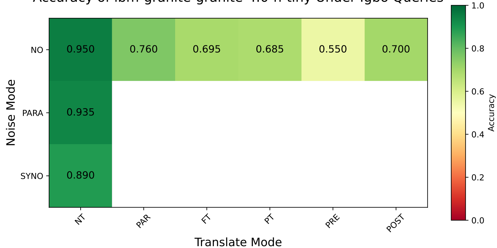
Accuracy of ibm-granite-granite-4.0-h-tiny Under Igbo Queries
