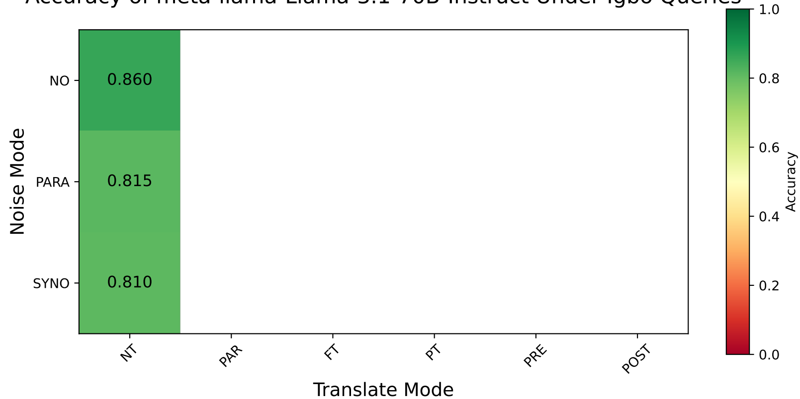
Accuracy of meta-llama-Llama-3.1-70B-Instruct Under Igbo Queries
