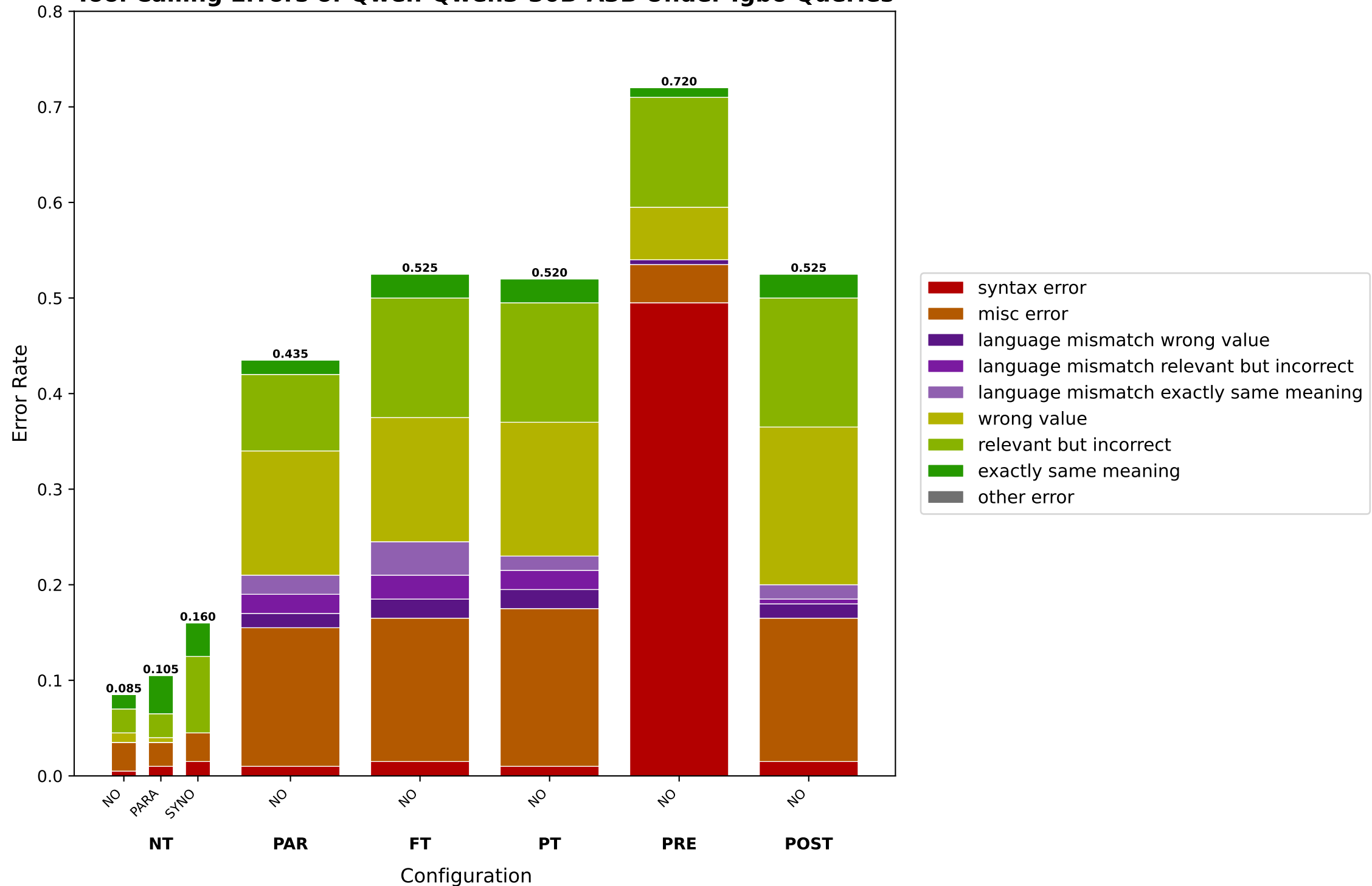
Tool Calling Errors of Qwen-Qwen3-30B-A3B Under Igbo Queries
