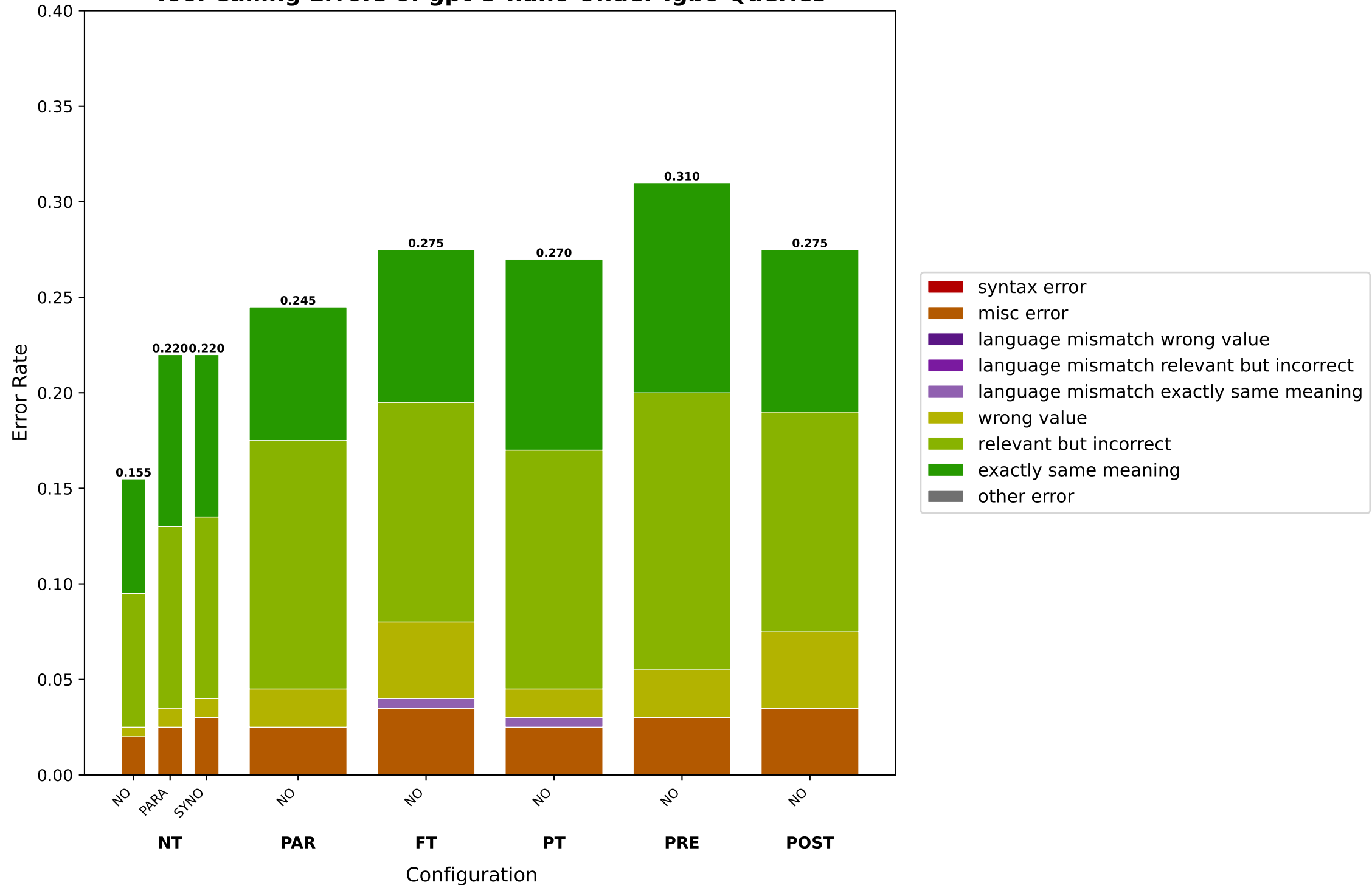
Tool Calling Errors of gpt-5-nano Under Igbo Queries
