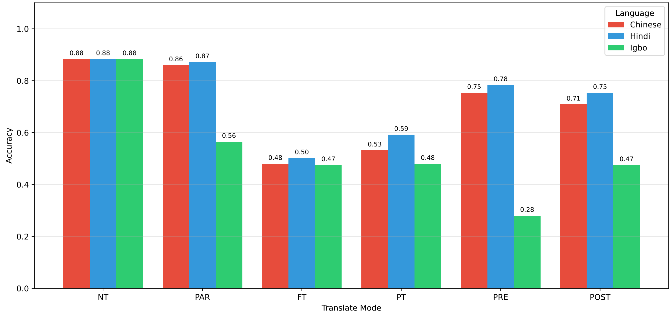
Qwen3-30B-A3B - Language Comparison
