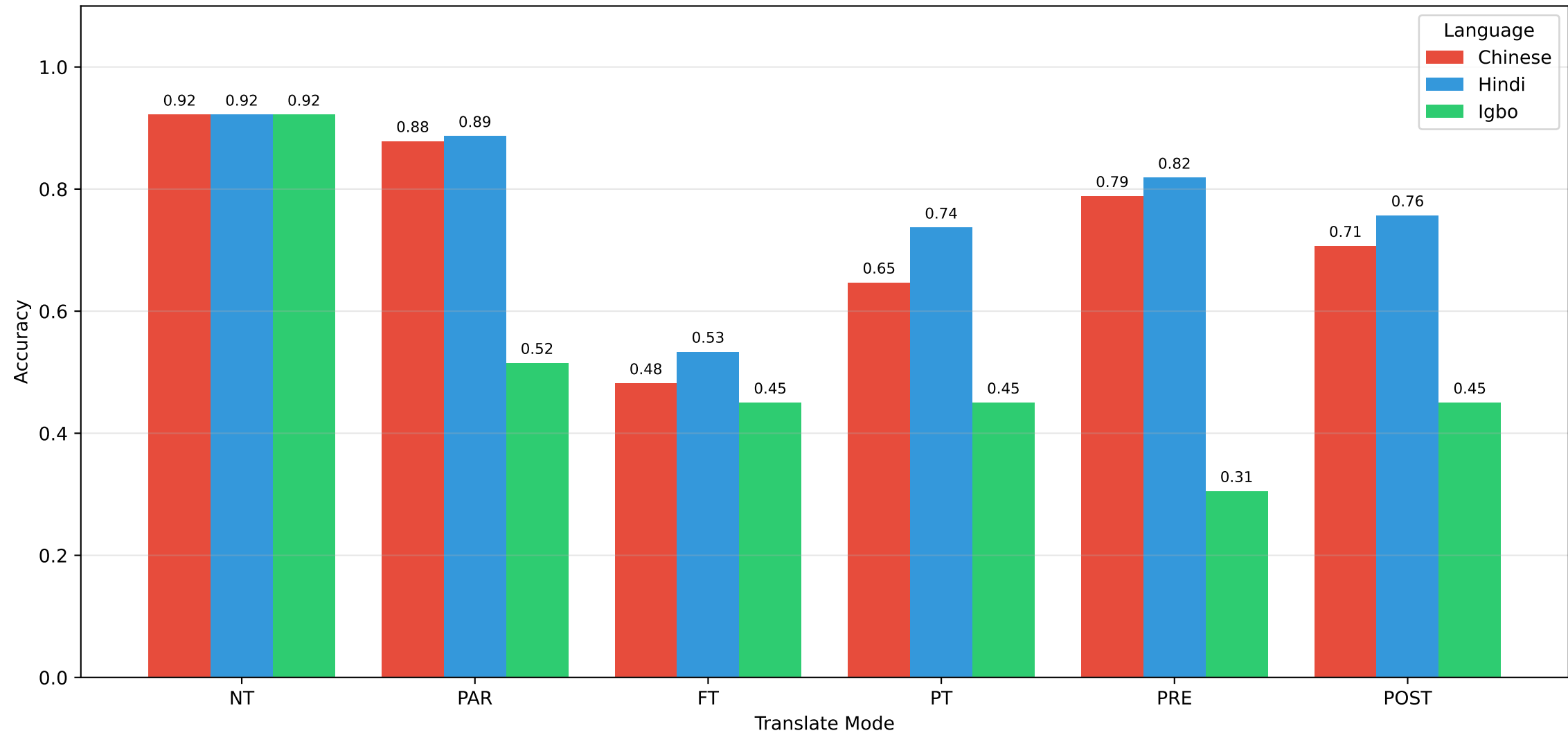
Qwen3-8B - Language Comparison
