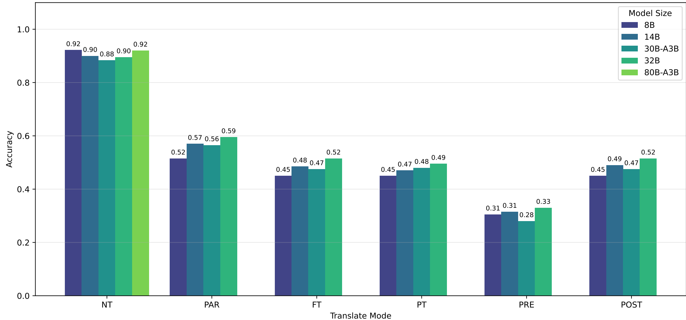
Qwen3 Model Size Comparison - Igbo
