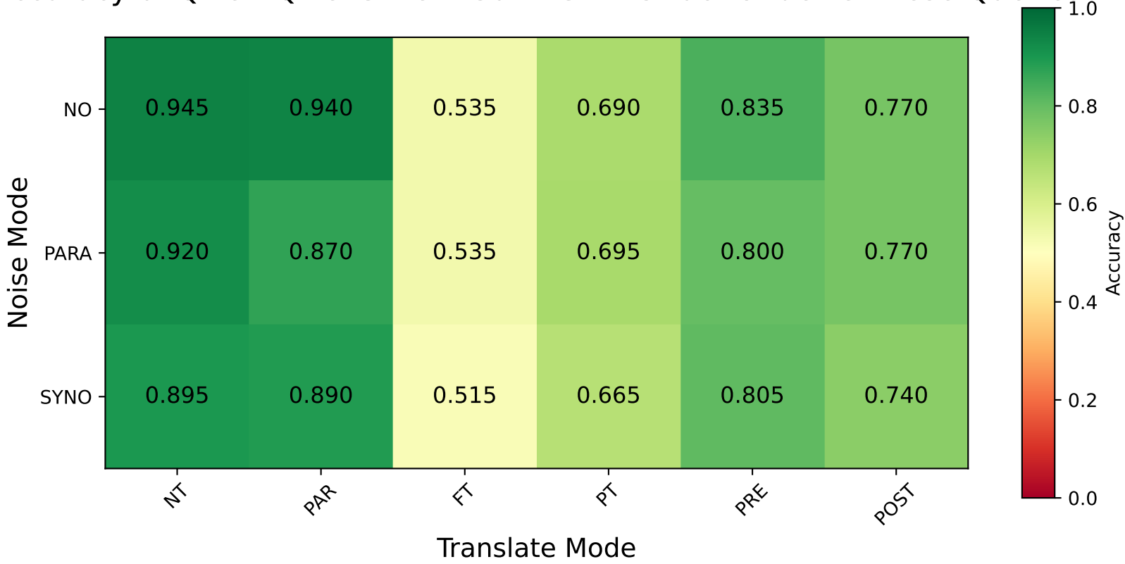
Accuracy of Qwen-Qwen3-Next-80B-A3B-Instruct Under Chinese Queries
