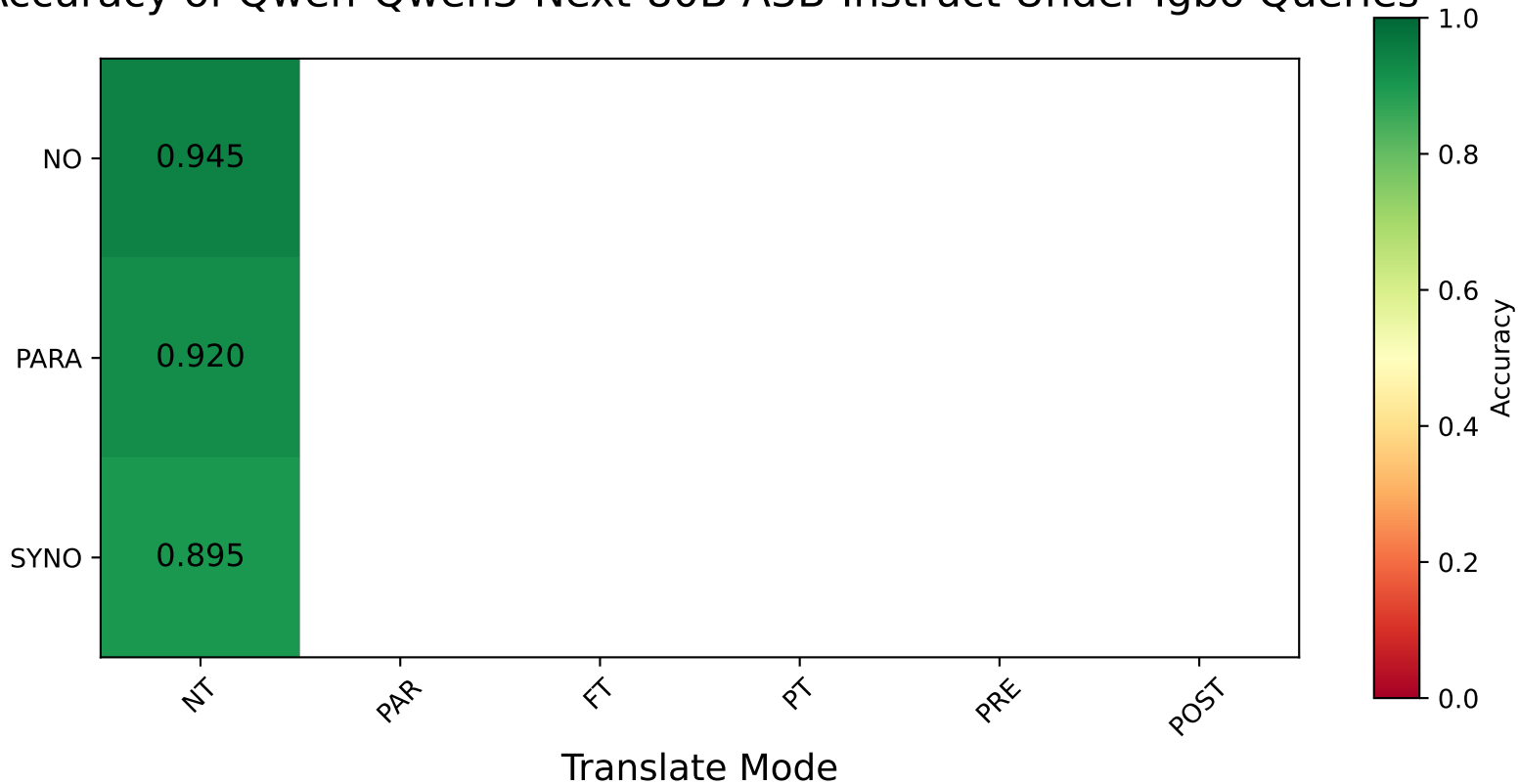
Accuracy of Qwen-Qwen3-Next-80B-A3B-Instruct Under Igbo Queries
