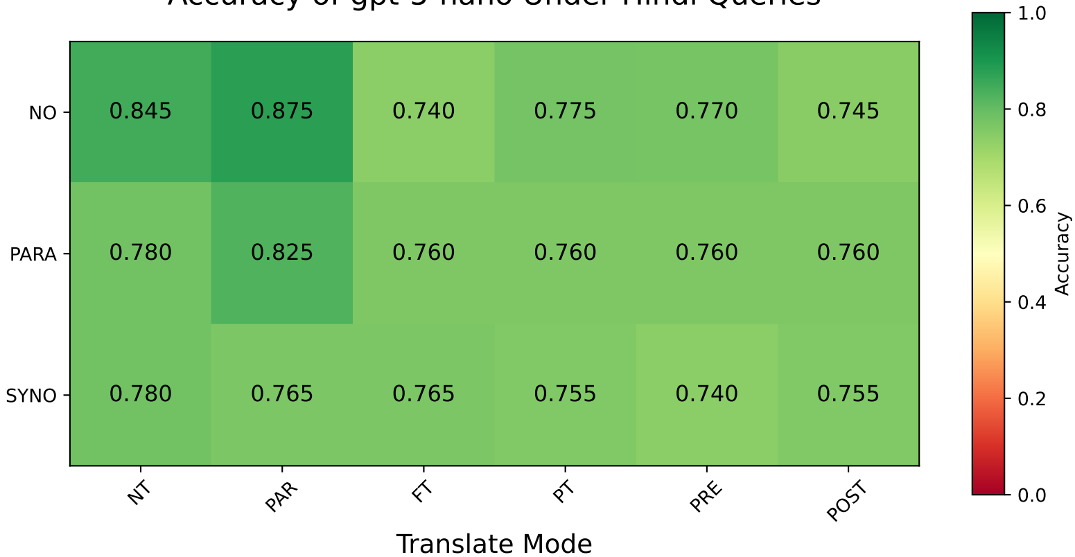
Accuracy of gpt-5-nano Under Hindi Queries
