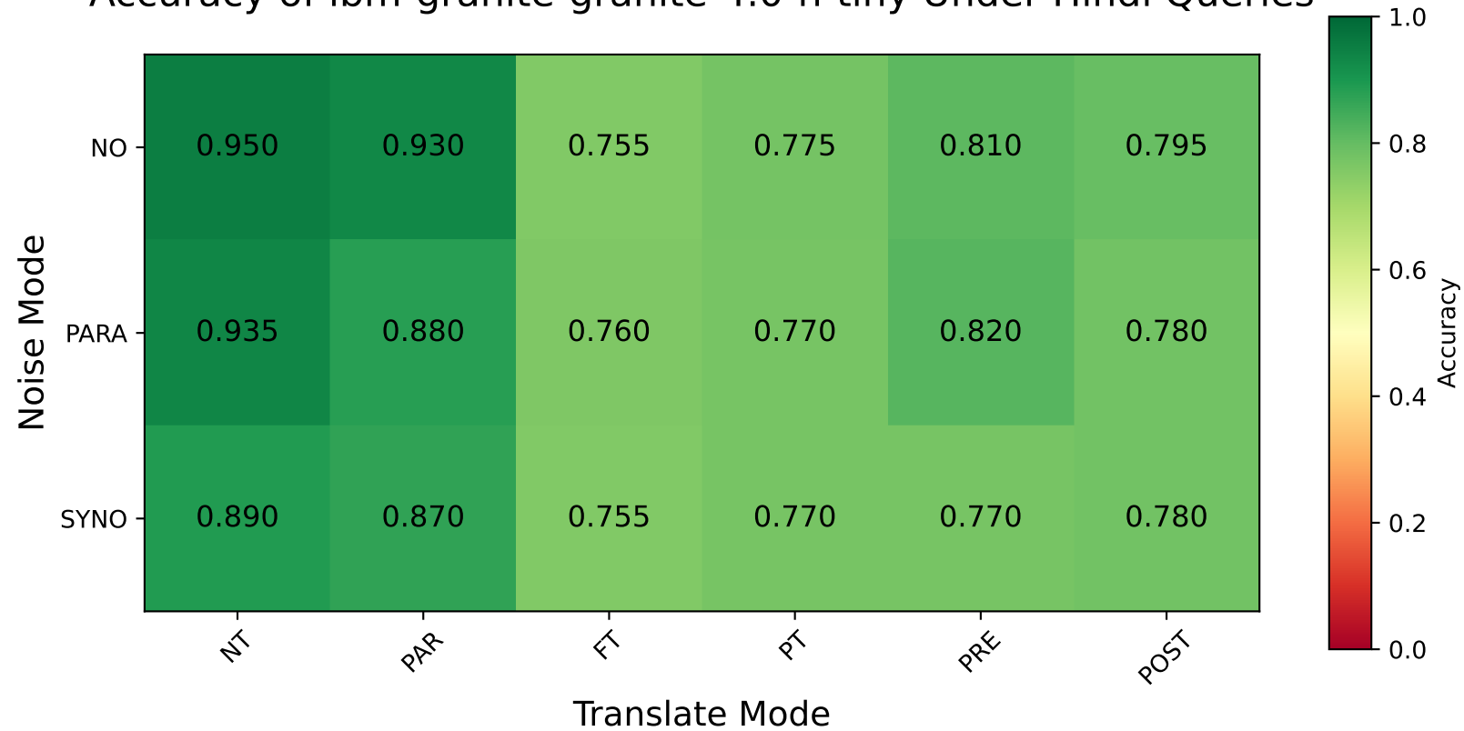
Accuracy of ibm-granite-granite-4.0-h-tiny Under Hindi Queries
