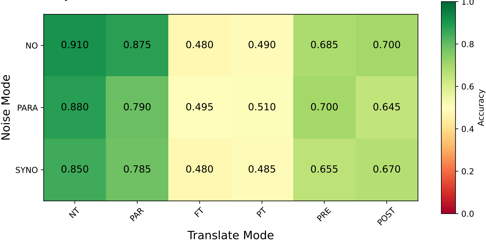
Accuracy of meta-llama-Llama-3.1-8B-Instruct Under Hindi Queries
