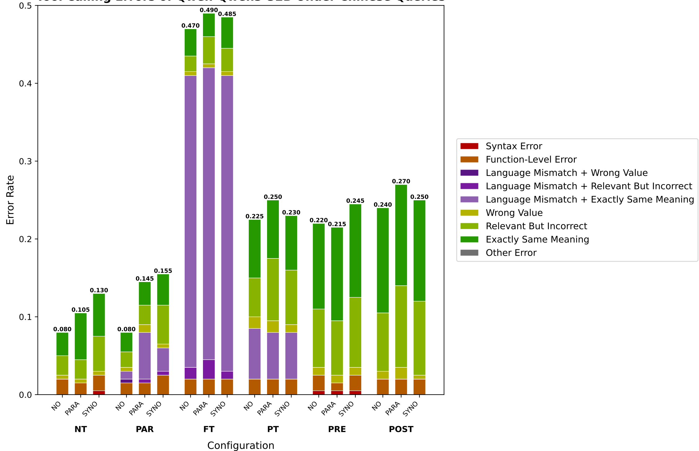
Tool Calling Errors of Qwen-Qwen3-32B Under Chinese Queries
