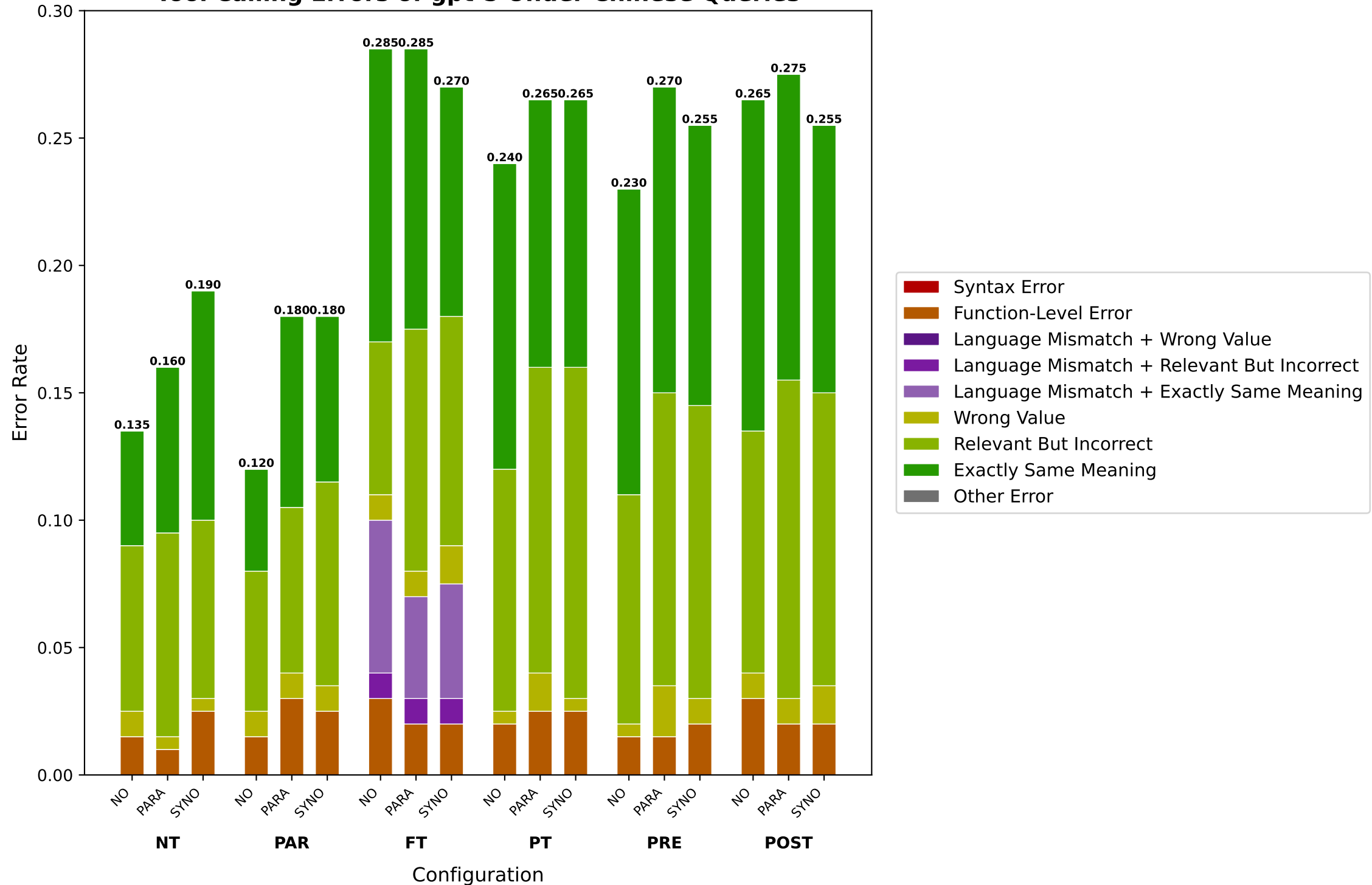
Tool Calling Errors of gpt-5 Under Chinese Queries
