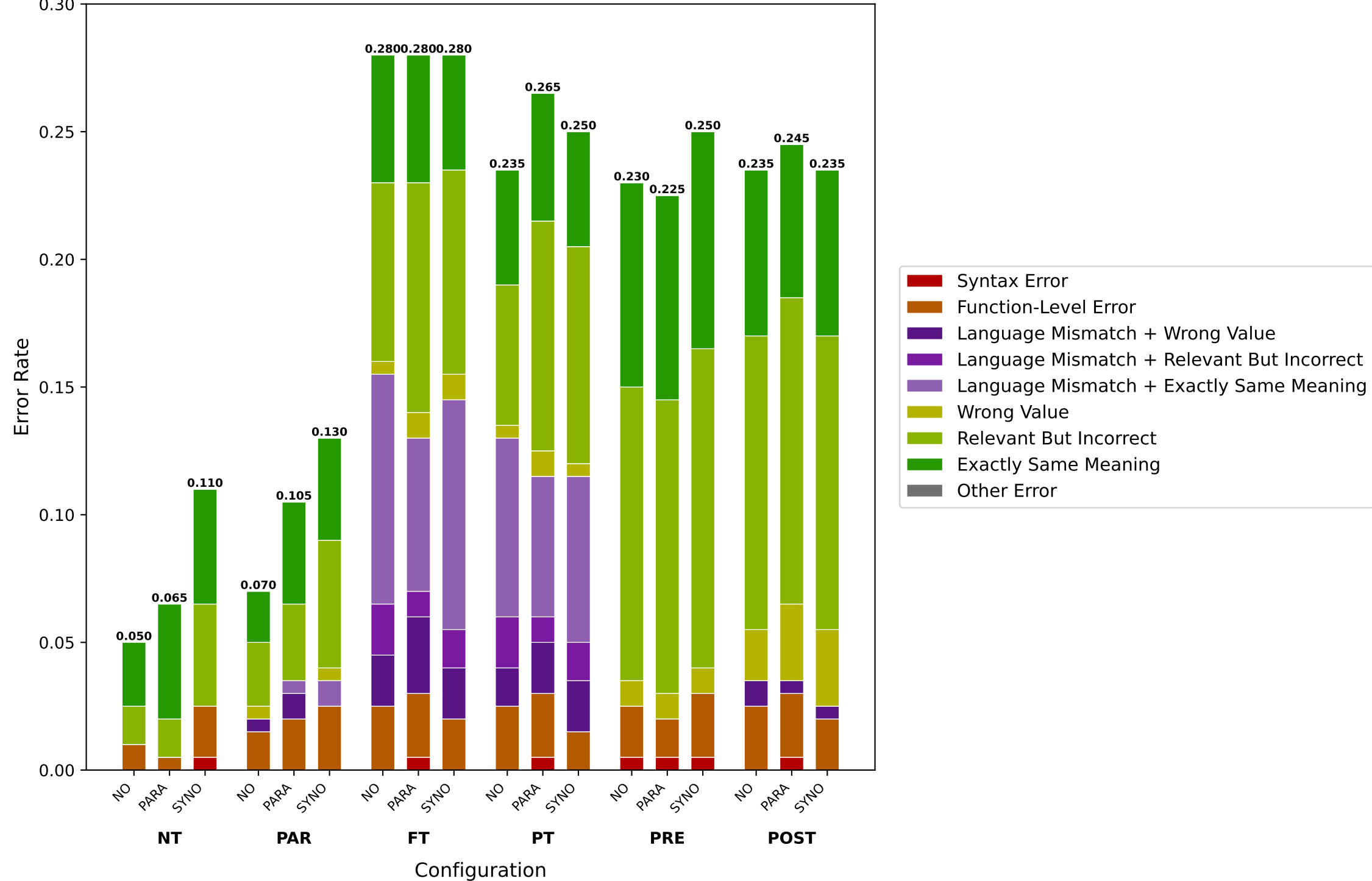
Tool Calling Errors of ibm-granite-granite-4.0-h-tiny Under Chinese Queries
