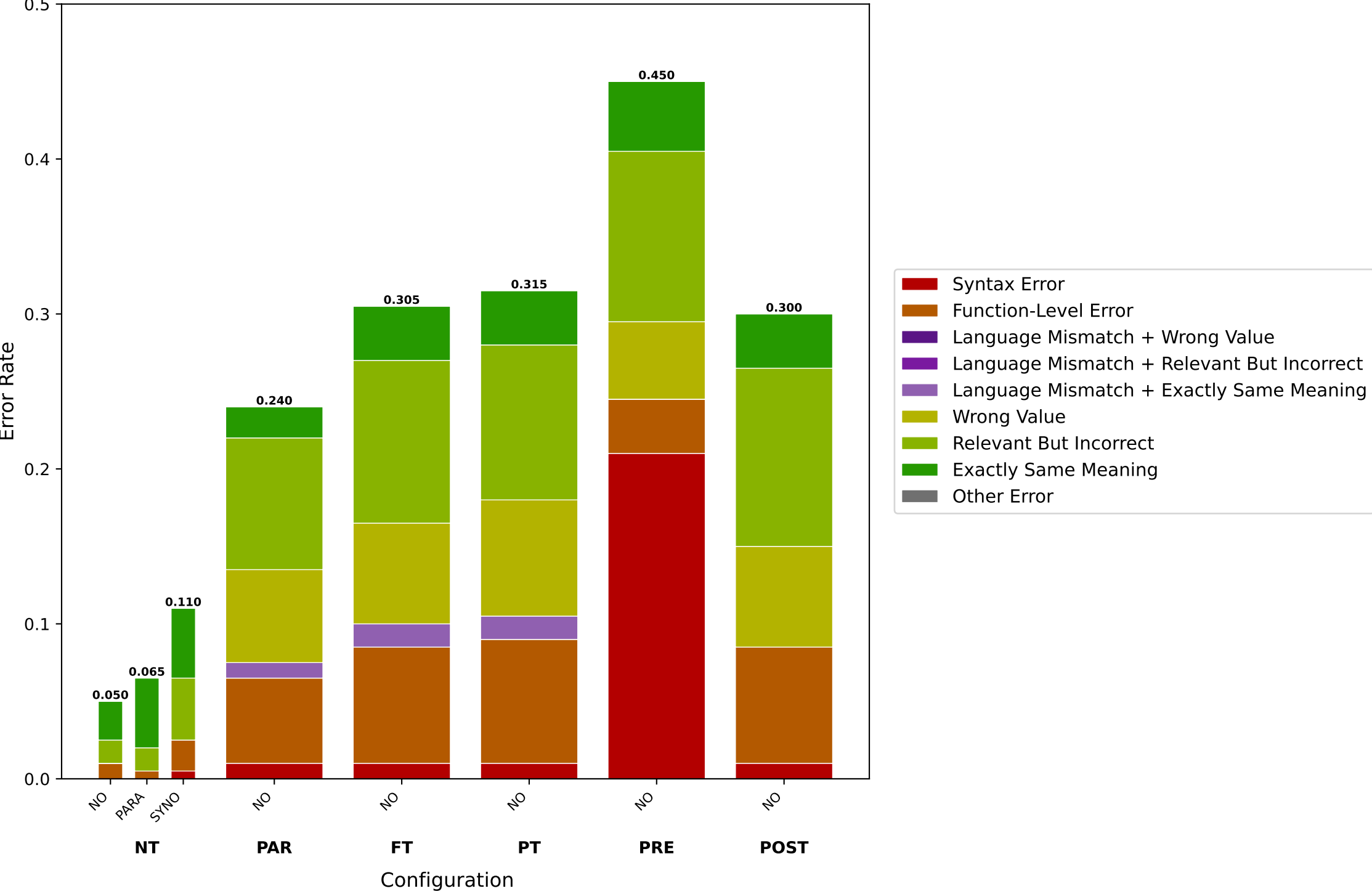
Tool Calling Errors of ibm-granite-granite-4.0-h-tiny Under Igbo Queries
