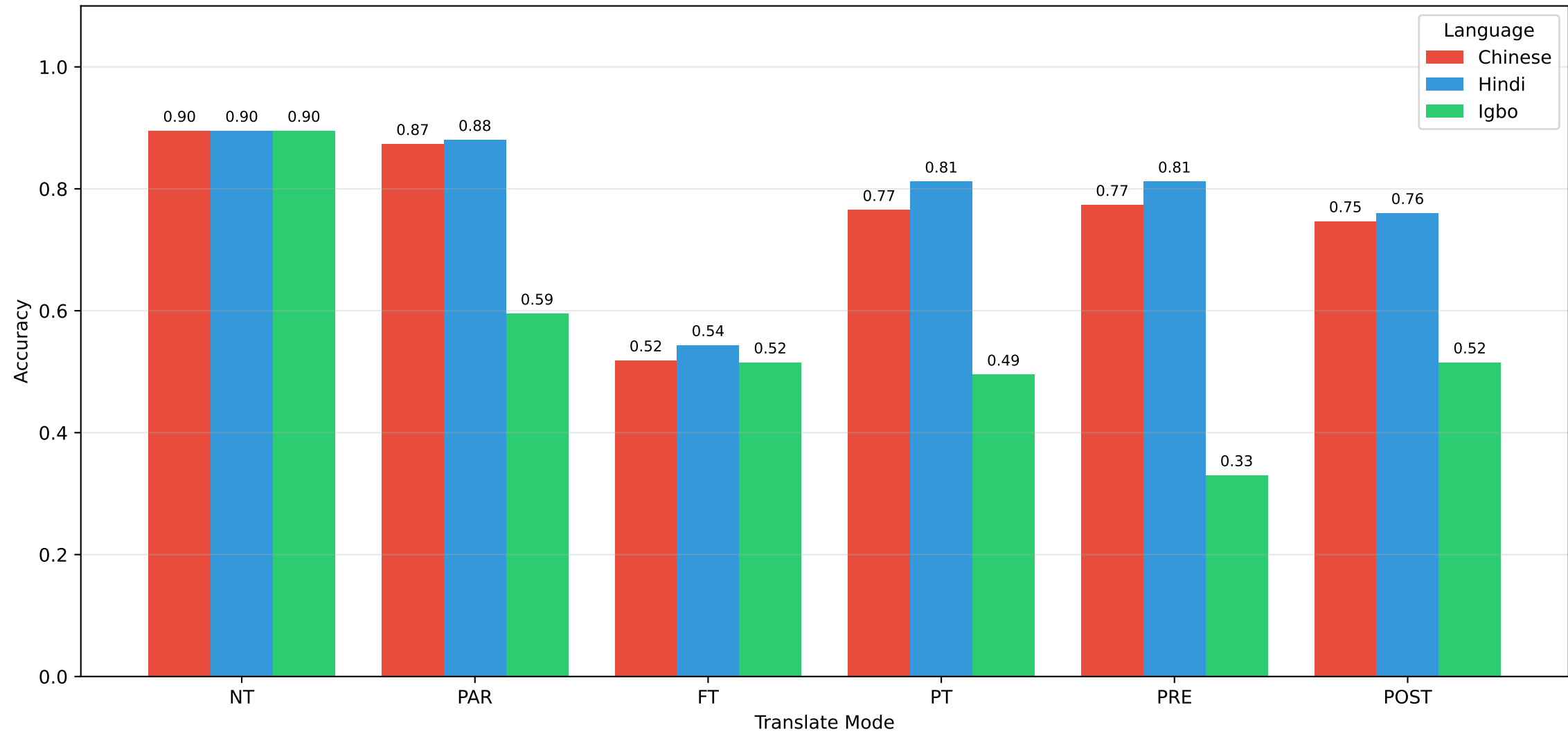
Qwen3-32B - Language Comparison
