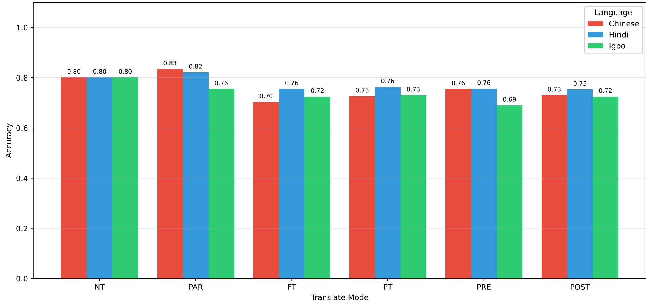
GPT-5 Nano - Language Comparison
