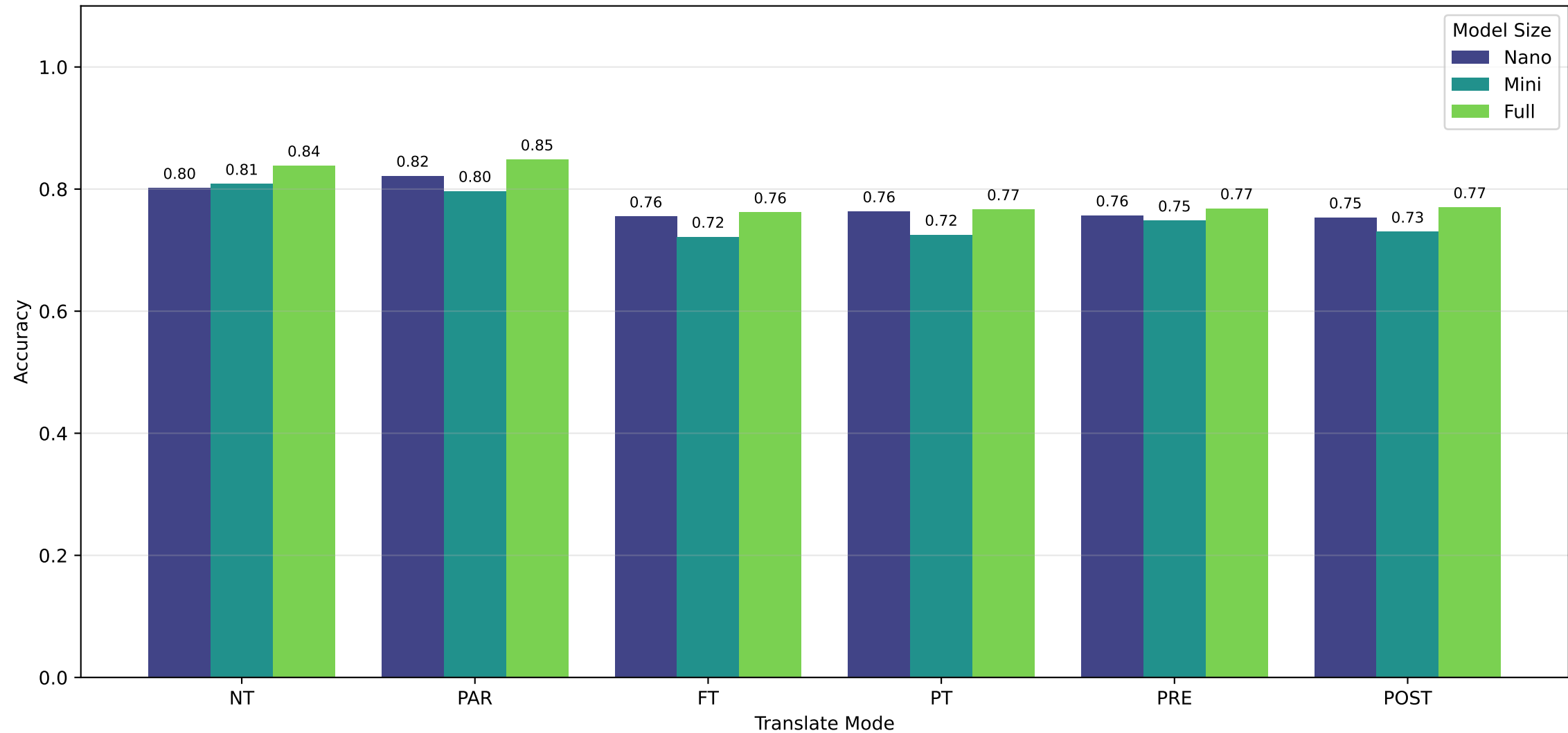
GPT-5 Model Size Comparison - Hindi
