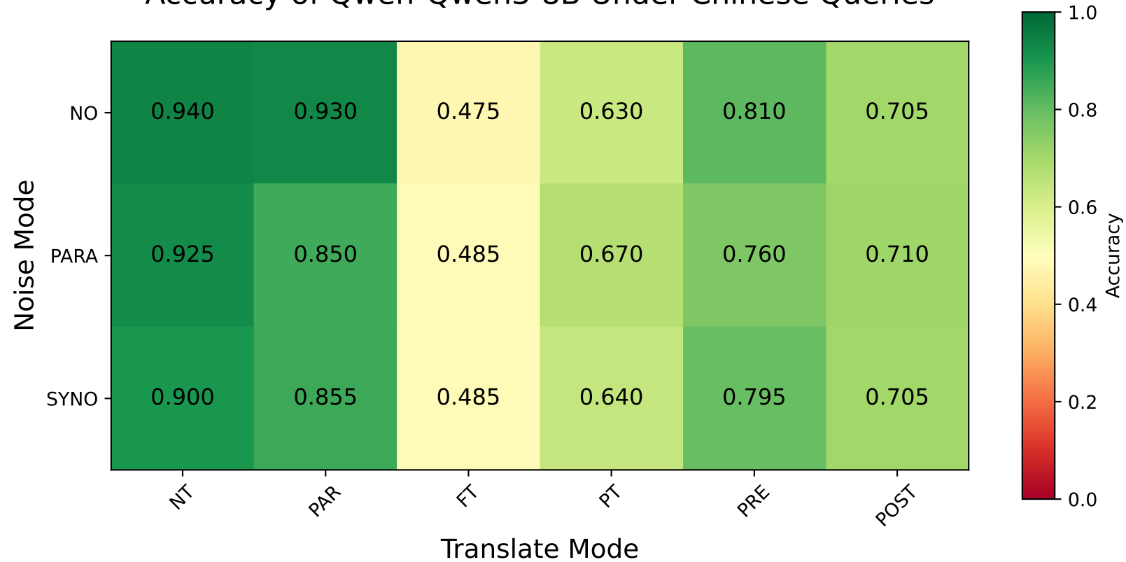
Accuracy of Qwen-Qwen3-8B Under Chinese Queries
