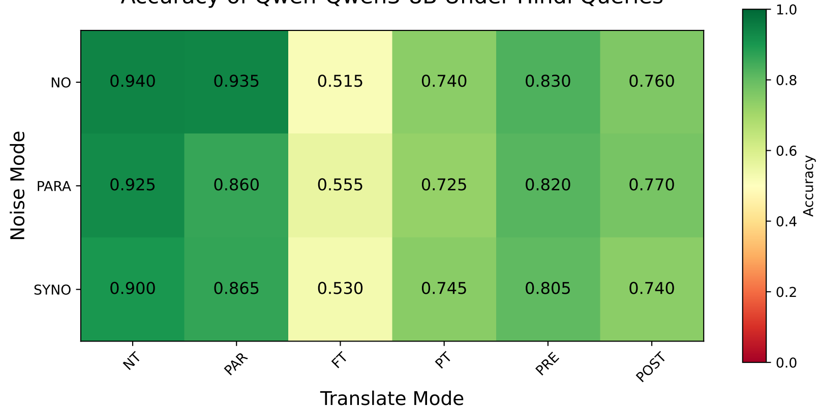
Accuracy of Qwen-Qwen3-8B Under Hindi Queries
