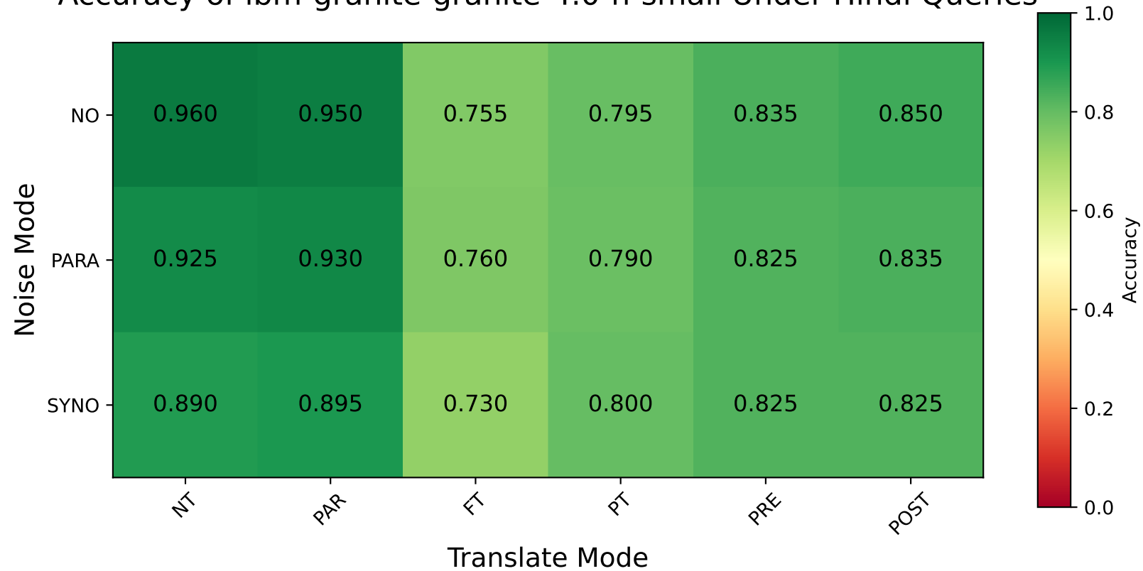
Accuracy of ibm-granite-granite-4.0-h-small Under Hindi Queries
