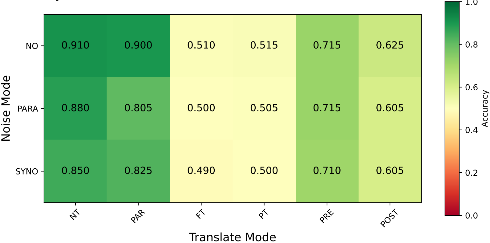
Accuracy of meta-llama-Llama-3.1-8B-Instruct Under Chinese Queries
