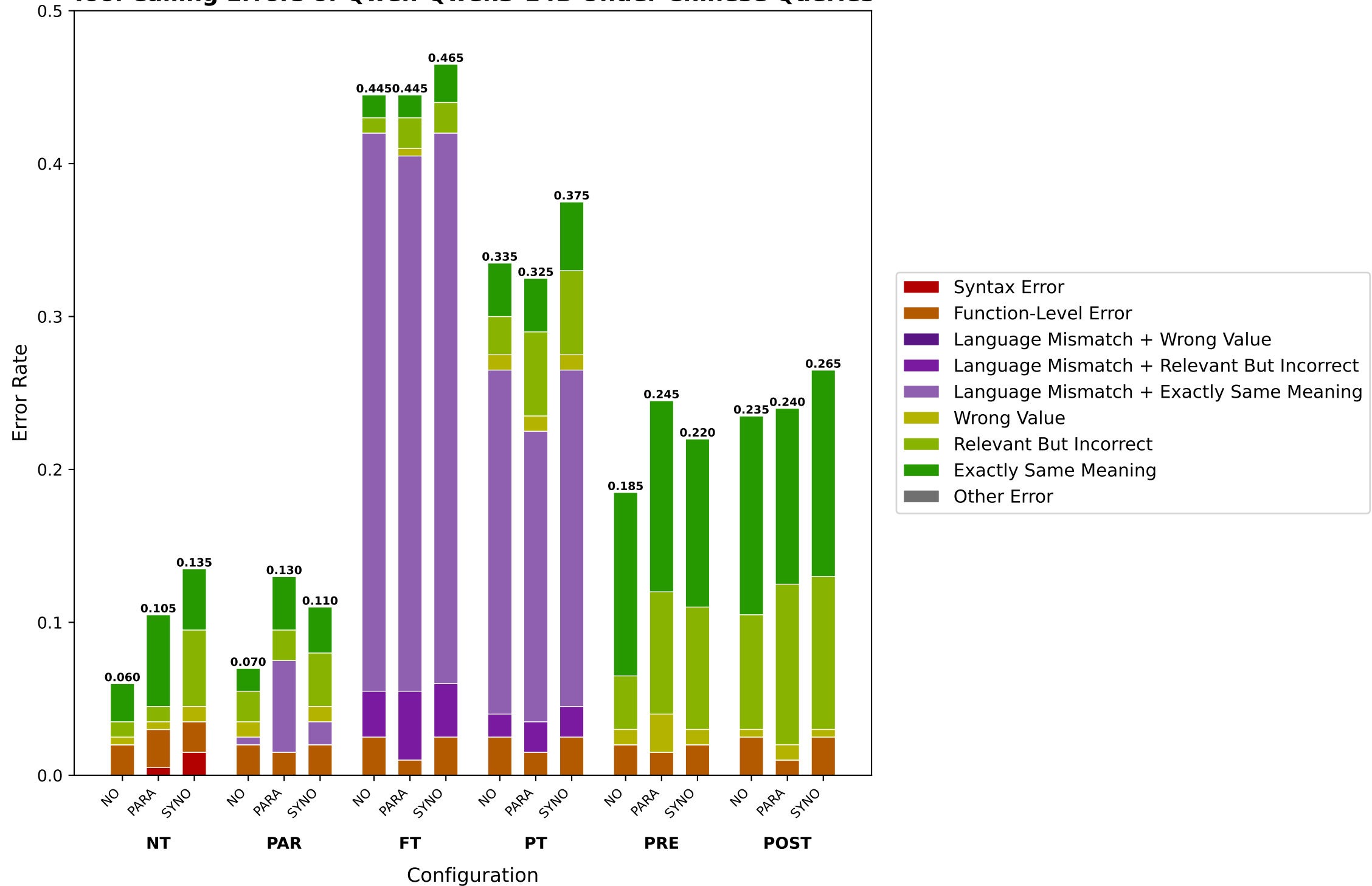
Tool Calling Errors of Qwen-Qwen3-14B Under Chinese Queries
