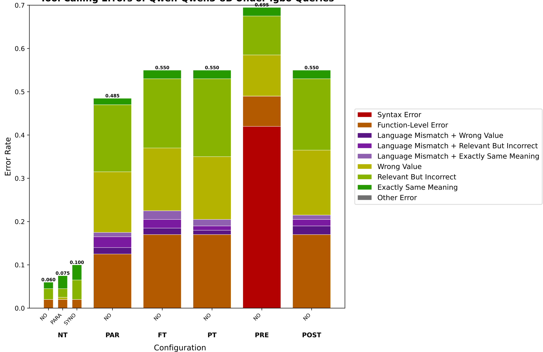
Tool Calling Errors of Qwen-Qwen3-8B Under Igbo Queries
