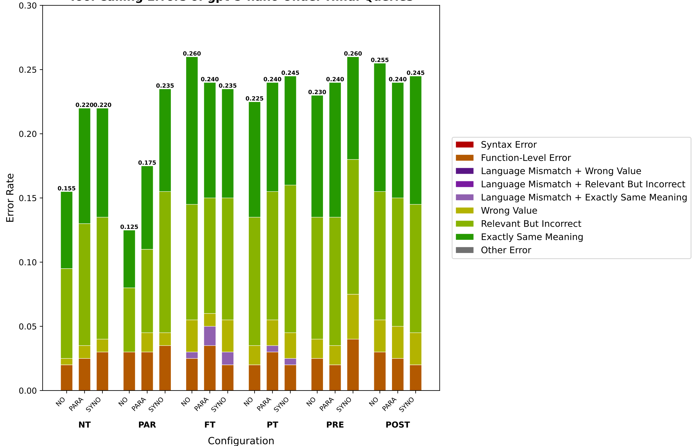
Tool Calling Errors of gpt-5-nano Under Hindi Queries
