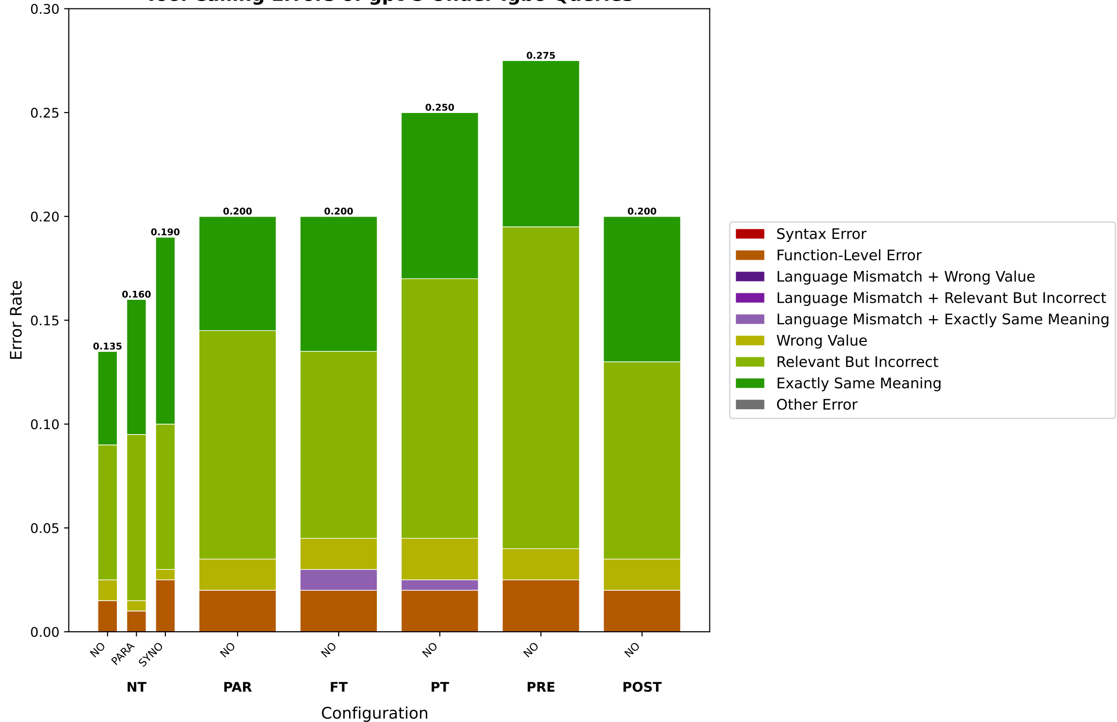
Tool Calling Errors of gpt-5 Under Igbo Queries
