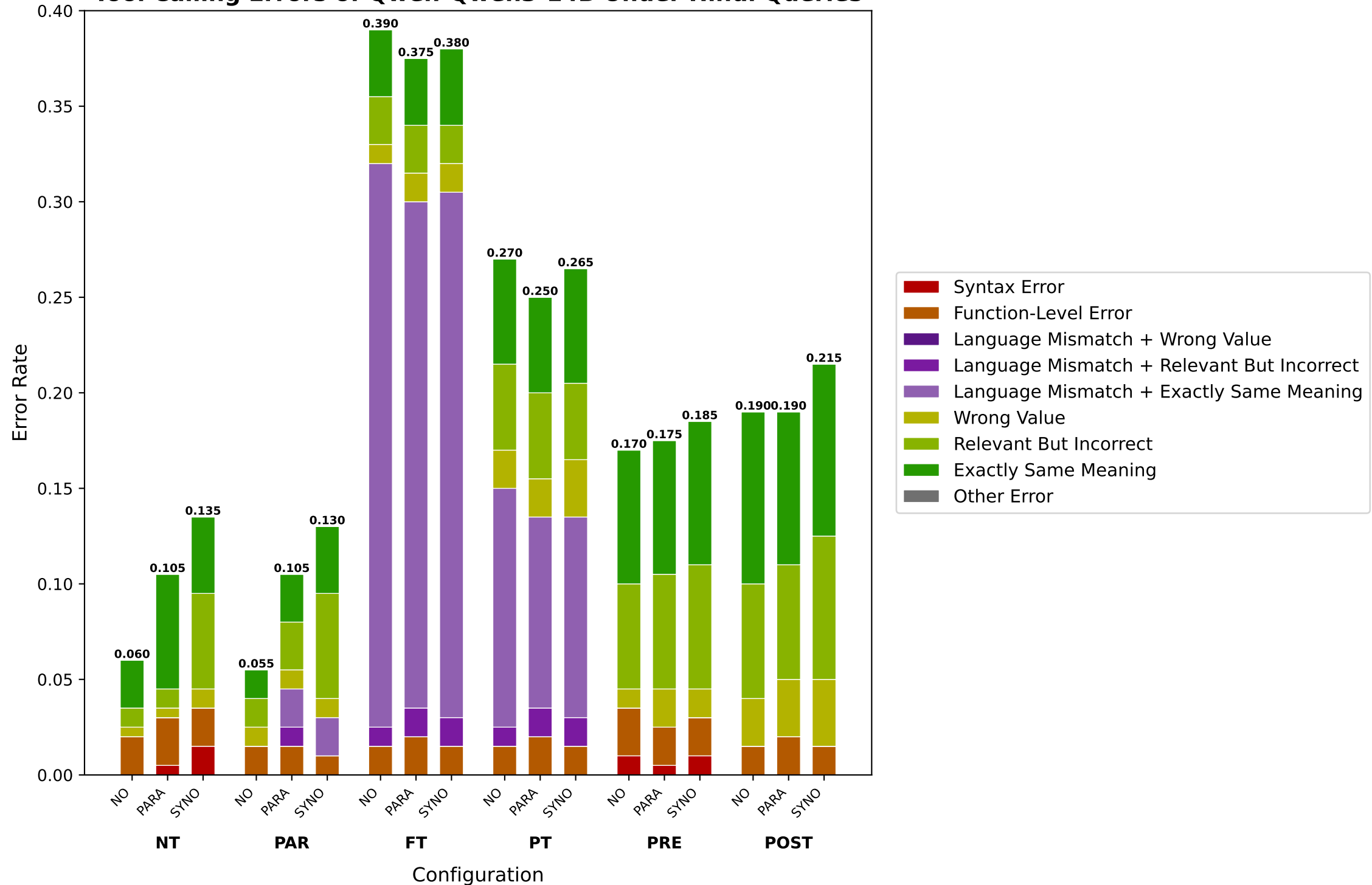
Tool Calling Errors of Qwen-Qwen3-14B Under Hindi Queries
