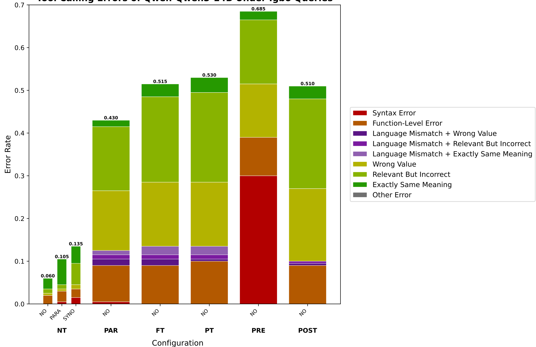
Tool Calling Errors of Qwen-Qwen3-14B Under Igbo Queries
