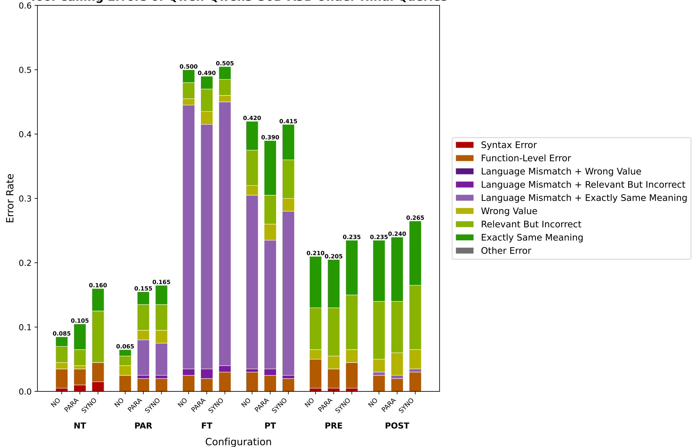
Tool Calling Errors of Qwen-Qwen3-30B-A3B Under Hindi Queries
