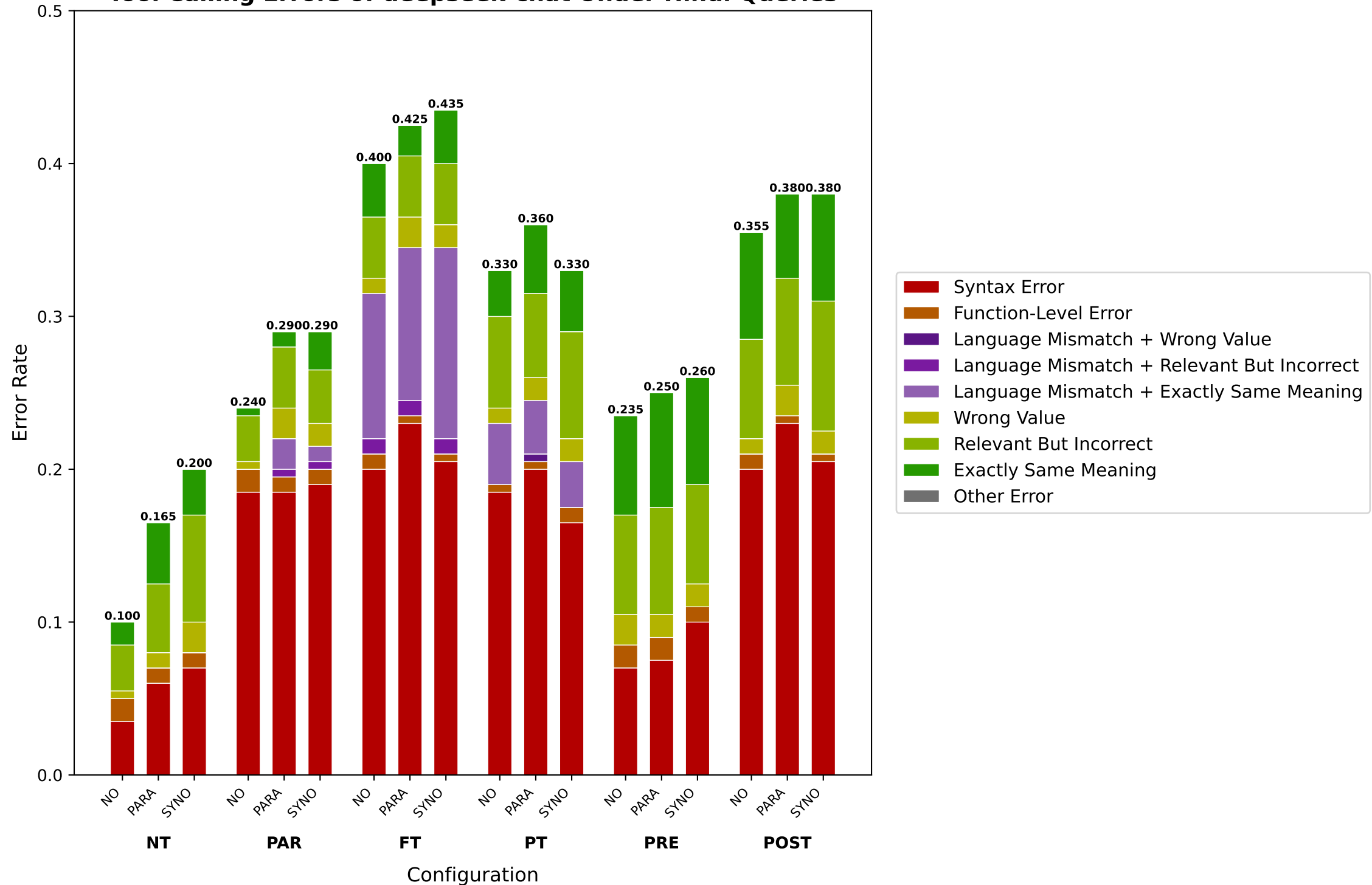
Tool Calling Errors of deepseek-chat Under Hindi Queries
