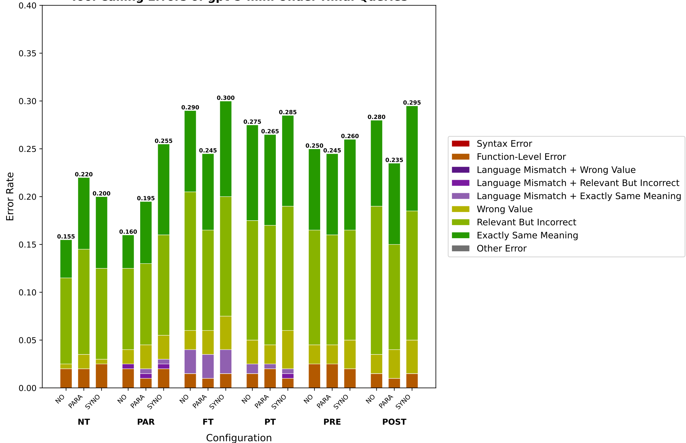
Tool Calling Errors of gpt-5-mini Under Hindi Queries
