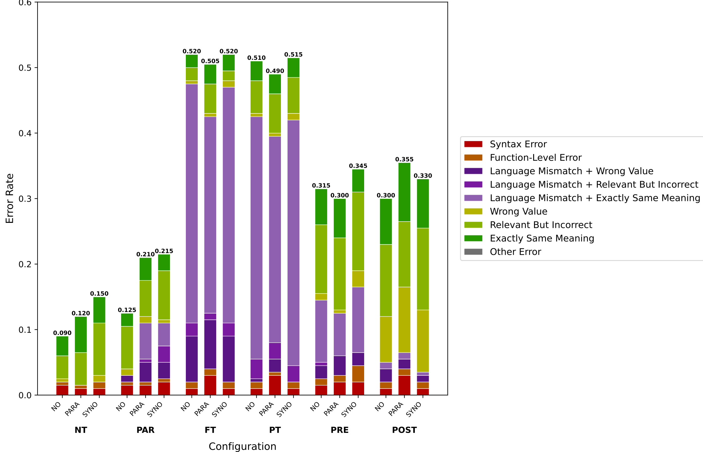
Tool Calling Errors of meta-llama-Llama-3.1-8B-Instruct Under Hindi Queries
