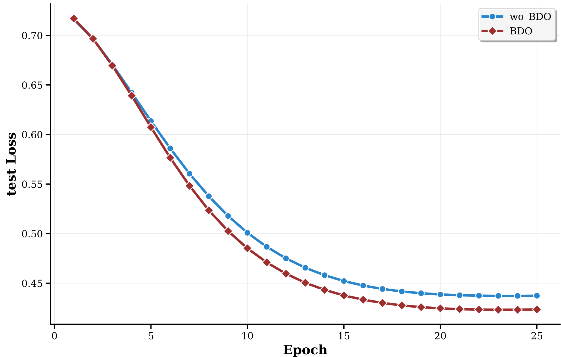
ETTh1 test Loss Comparison
