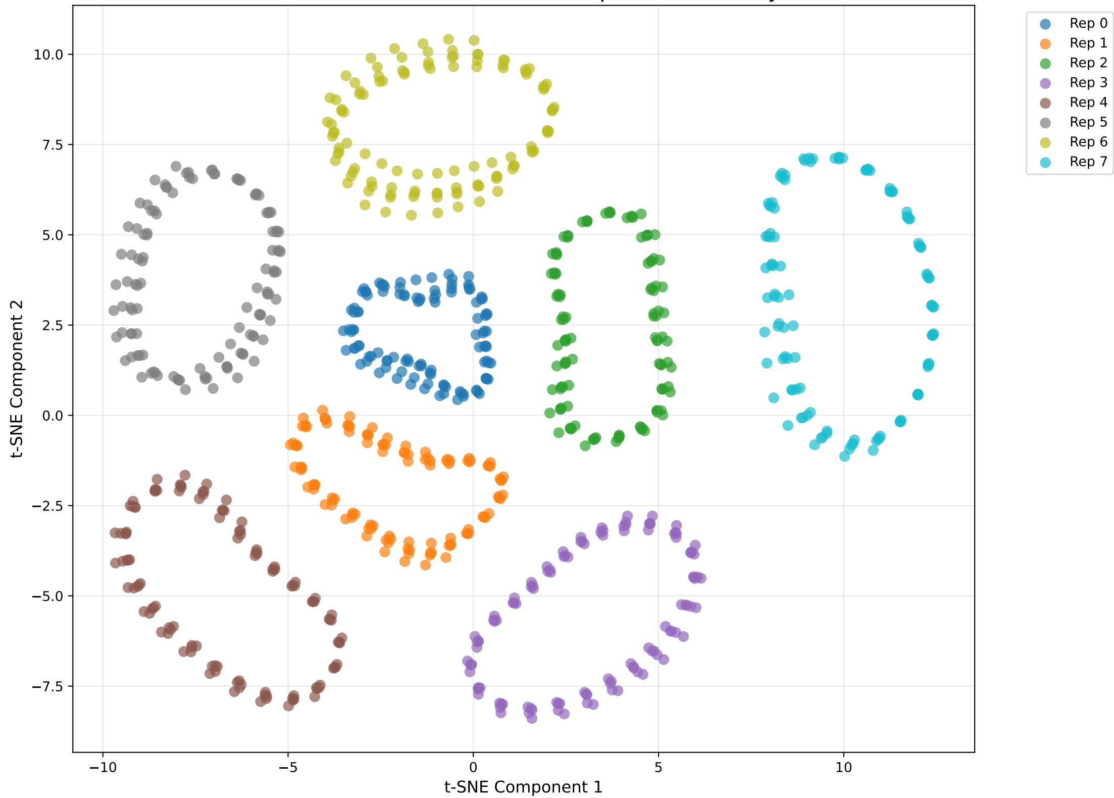
t-SNE Visualization of Different Representation Layers
