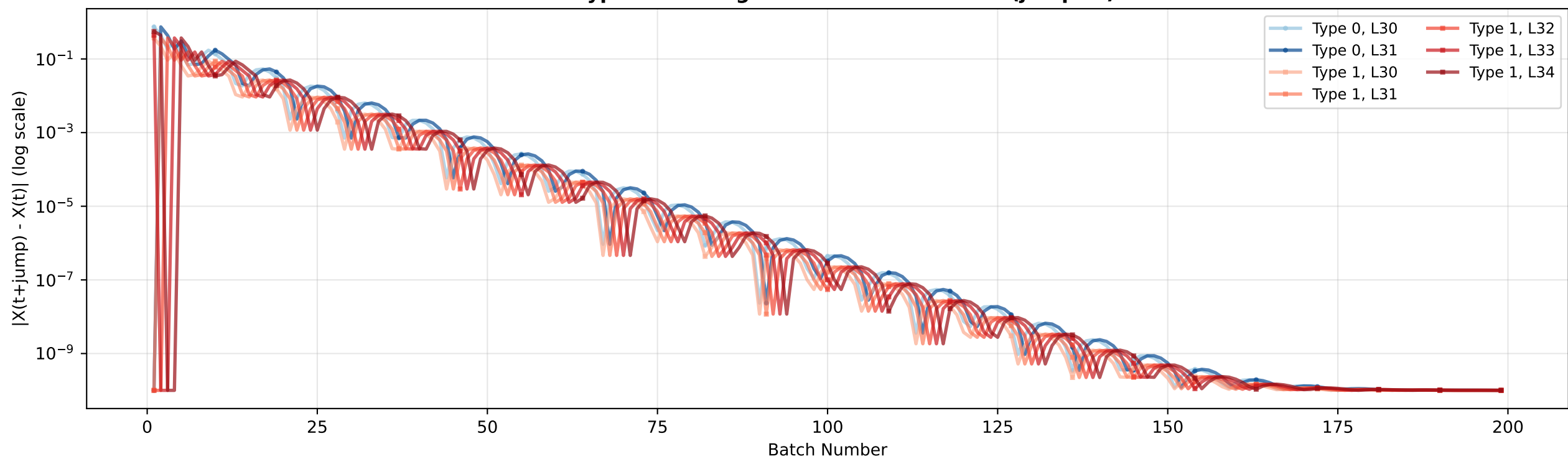
All Types and Lengths - State Differences (jump=1)
