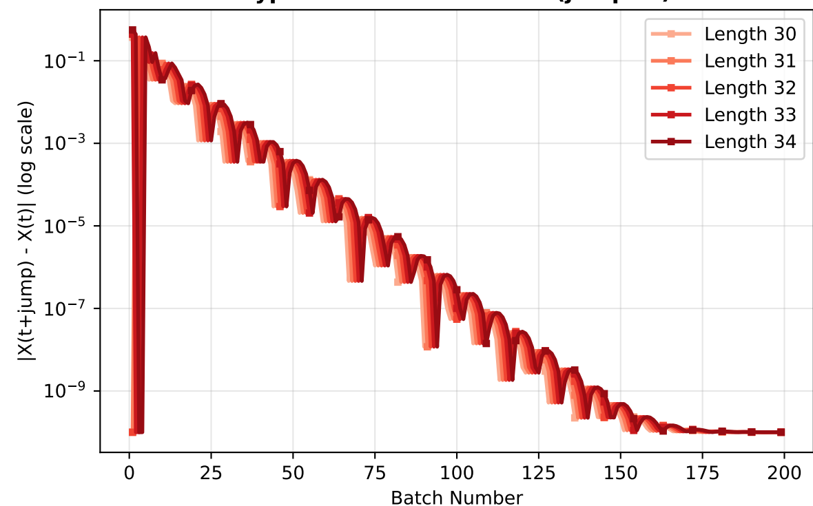
Type 1 State Differences (jump=1)
