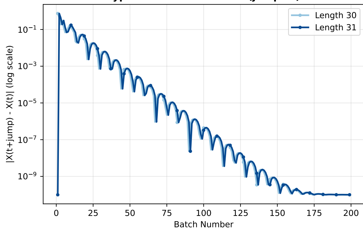
Type 0 State Differences (jump=1)
