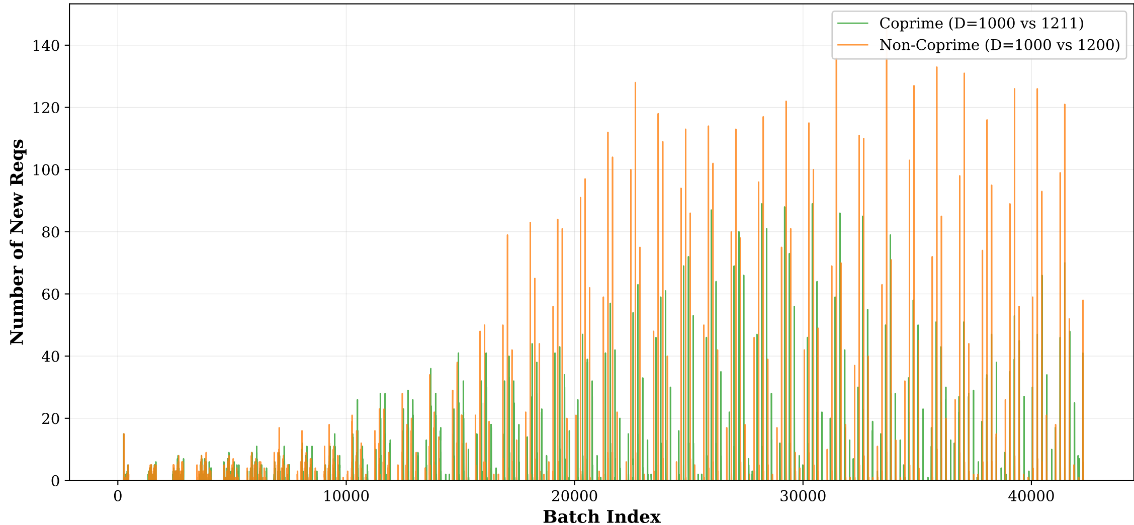
Admission: Coprime vs Non-Coprime (P=5000)
