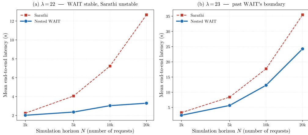
Figure 10 Long-horizon check near the transition from near-overloaded to overloaded on (0.7p512d20, 0.3p512d50). At \lambda = 22 , Nested WAIT approaches a finite latency plateau while Sarathi grows rapidly with N ; at \lambda = 23 , both policies show continued latency growth, but Nested WAIT remains lower-latency.
