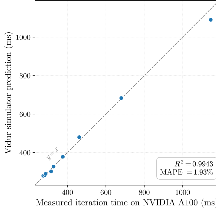
Figure 18 Simulator calibration against NVIDIA A100 80 GB GPU measurements. Each marker is one batch-size configuration: its horizontal coordinate is the measured GPU batch inference time, and its vertical coordinate is the Vidur prediction. The comparison uses prefill length 256 and decode length 20 while varying B over the grid \{1, 2, 4, \dots, 256\} . The dashed line is the y = x reference. The fitted linear iteration-time model in Equation (1) achieves R^2 = 0.9943 and mean absolute percentage error 1.93% on the plotted grid.
