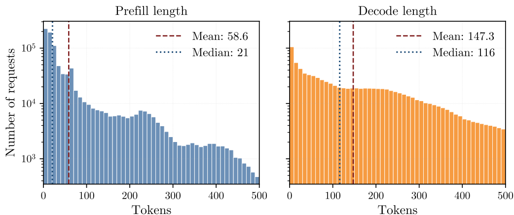
Figure 11 Filtered prompt-length distributions in lmsys-chat-1m : prefill lengths on the left and decode lengths on the right, restricted to requests with both lengths below 500 tokens. The dashed lines mark the mean and median of each distribution.
