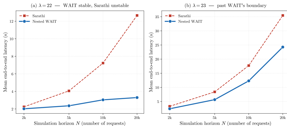
Figure 10 Long-horizon validation on (0.7p512d20, 0.3p512d50). At \lambda = 22 , Nested WAIT approaches a finite latency plateau while Sarathi grows with N ; at \lambda = 23 , both policies are unstable, but Nested WAIT remains lower-latency.
