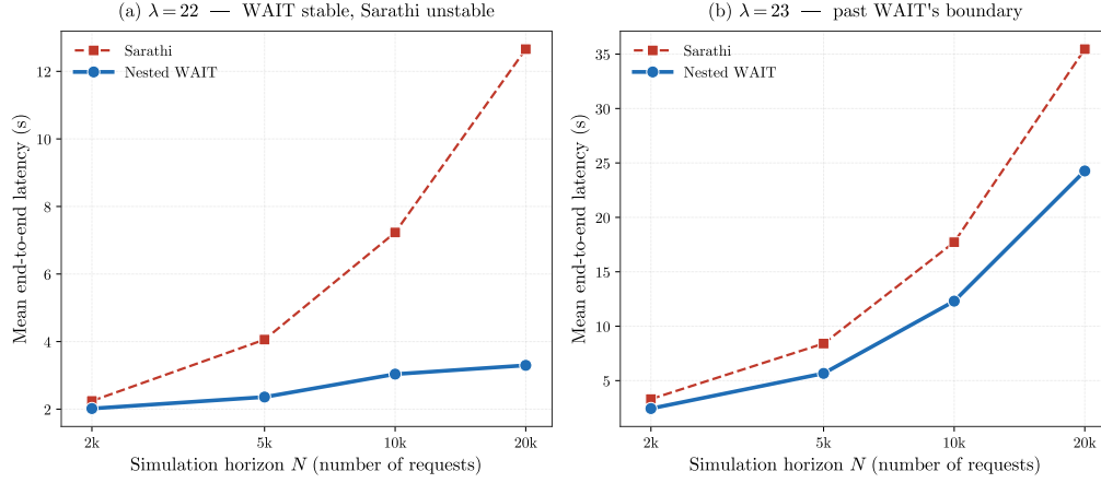
Figure 10 Long-horizon check near the transition from near-overloaded to overloaded on (0.7\text{p512d20}, 0.3\text{p512d50}) . At \lambda = 22 , Nested WAIT approaches a finite latency plateau while Sarathi grows rapidly with N ; at \lambda = 23 , both policies show continued latency growth, but Nested WAIT remains lower-latency.
