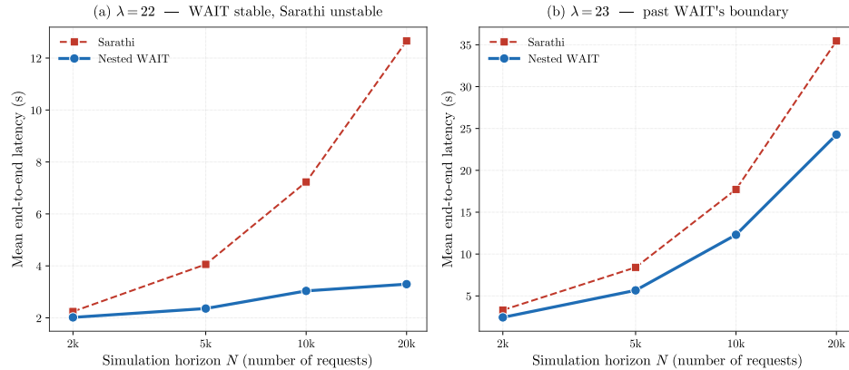
Figure 10 Long-horizon check near the transition on (0.7\text{p512d20}, 0.3\text{p512d50}) . At \lambda = 22 , Nested WAIT approaches a finite latency plateau; at \lambda = 23 , both policies show continued latency growth, but Nested WAIT remains lower-latency.
